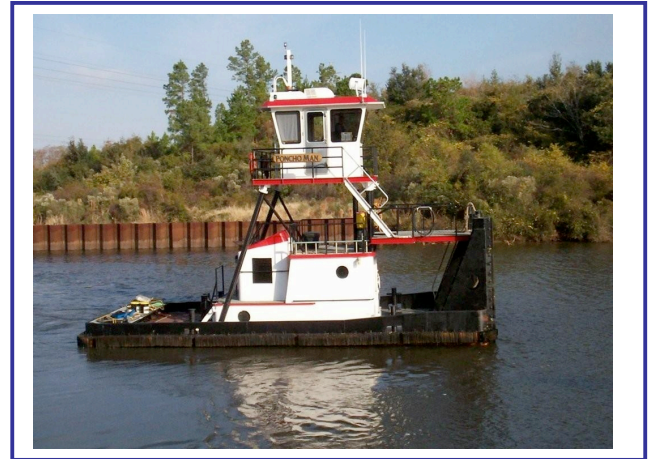
1052 HP Inland Push Boat
